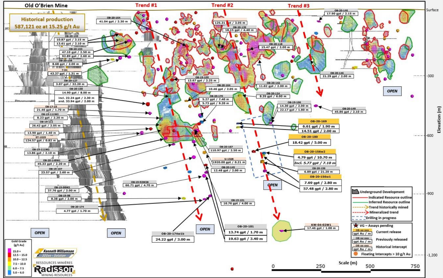
O'Brien Project - MRE2019* Indicated and Inferred Resource distribution @ 5.0 g/t Au cut-off Longitudinal Vertical Section – Looking North
